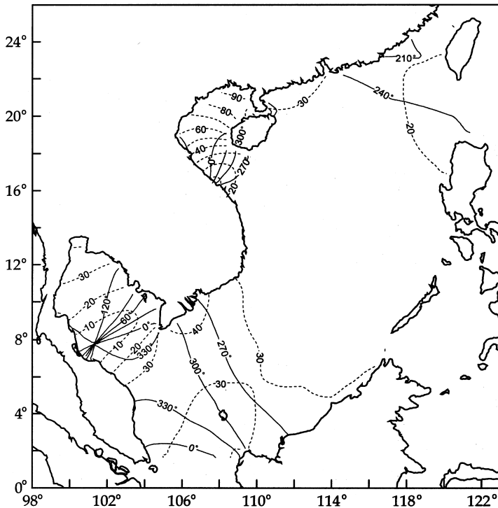
Fig. 6. As in Fig. 3 but for O_1 .
